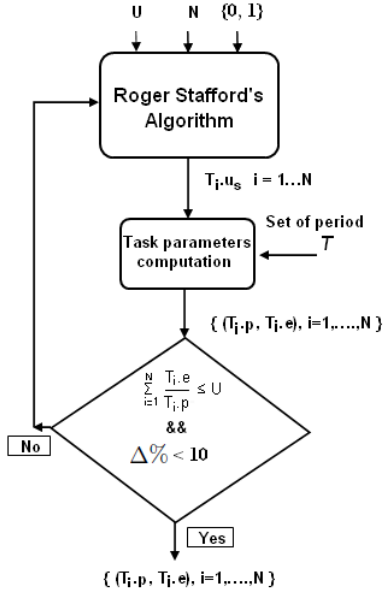
Figure 3. Dataset generator
