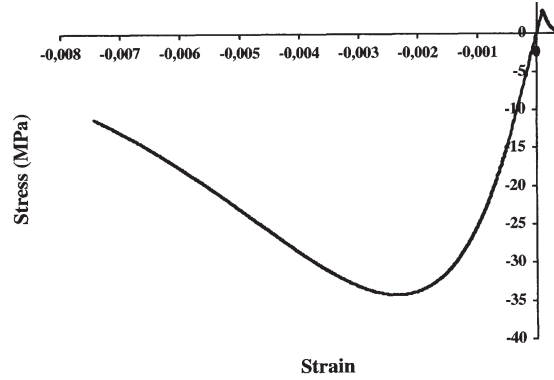
Figure 3. Simulation of the uniaxial (tension and compression) response of a concrete. From (Pijaudier-Cabot and Mazars, 2001)
