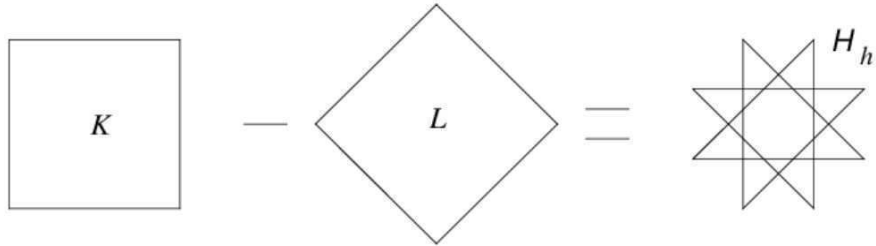
Figure 2. The Minkowski difference K - L (polytopal case)
