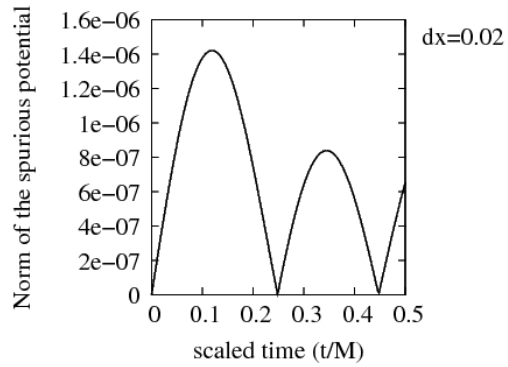
Fig. 8: \|\mathbf{u}_h^\perp\|(t) when 0 \leq t/M \leq 0.5 All Mach Godunov scheme
