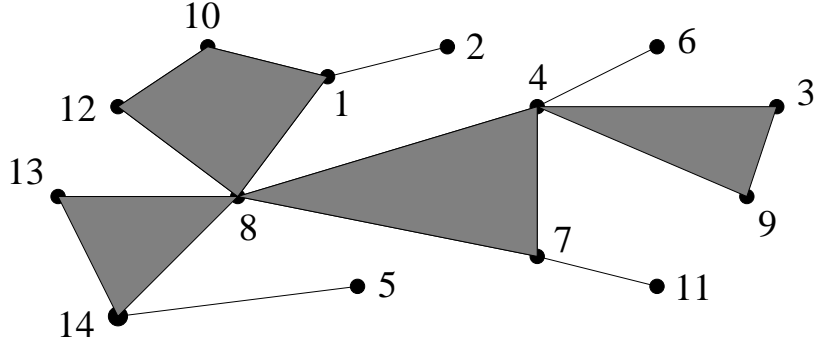
Figure 1: A hypertree
