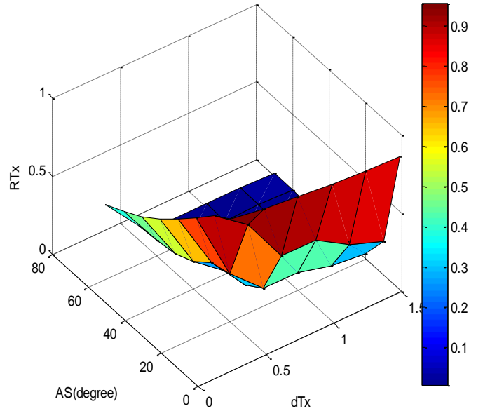
Figure 6: R_{Tx} versus Angular Spread and transmitting antennas spacing ( d_{Tx} )
