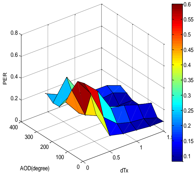
Figure 8: PER versus Angle of Departure and spacing of transmitting antenna ( d_{Tx} in \lambda )
