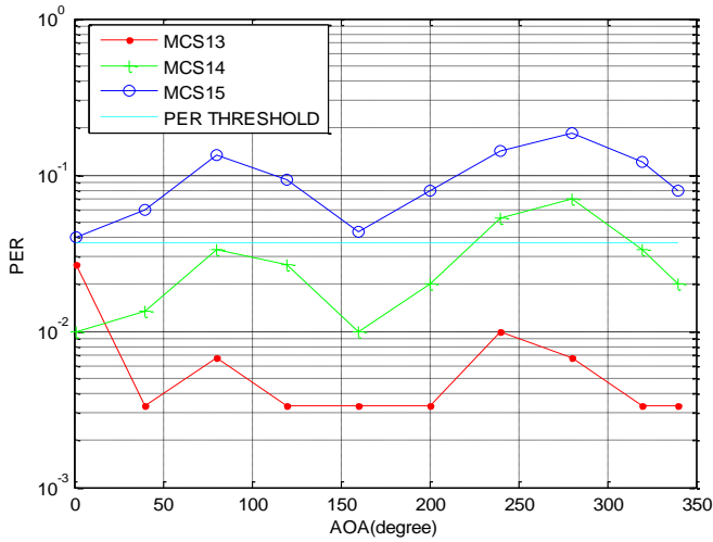
Figure 5: PER versus Angle of Arrival (AOA) for MCS13, 14 and 15. Channel D, SNR = 38 dB
