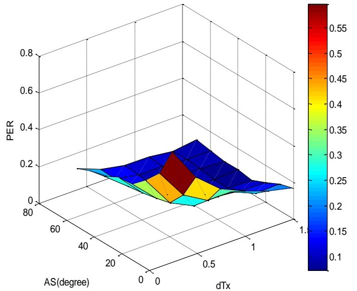
Figure 7: PER versus Angular Spread and transmitting antennas spacing ( d_{Tx} )
