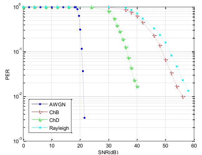
Figure 2: Simulated PER versus SNR for reference wireless channels
