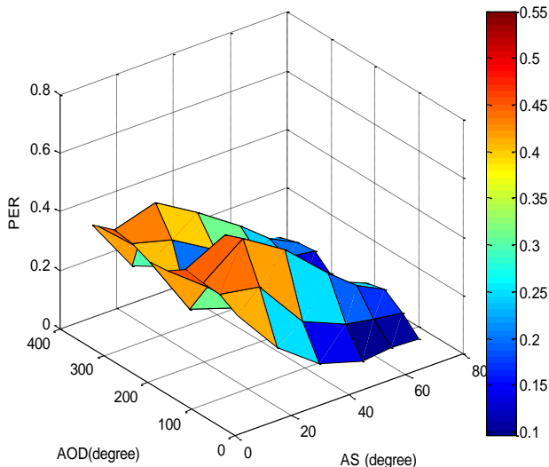
Figure 9: PER versus Angle of arrival and Angular Spread
