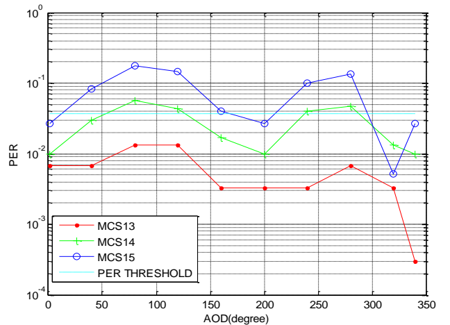
Figure 4: PER versus Angle of Departure (AOD) for MCS13, 14 and 15. Channel D, SNR = 38 dB
