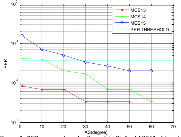
Figure 3: PER versus Angular Spread (AS) for MCS13, 14 and 15. Channel D, SNR = 38 dB
