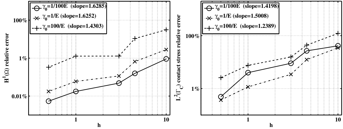
Figure 6: Convergence in the 2D case with P_2 elements and \theta = 0 . Left : relative H^1(\Omega) -norm on the displacements. Right : relative weighted L^2(\Gamma_C) -norm on the contact pressure.
