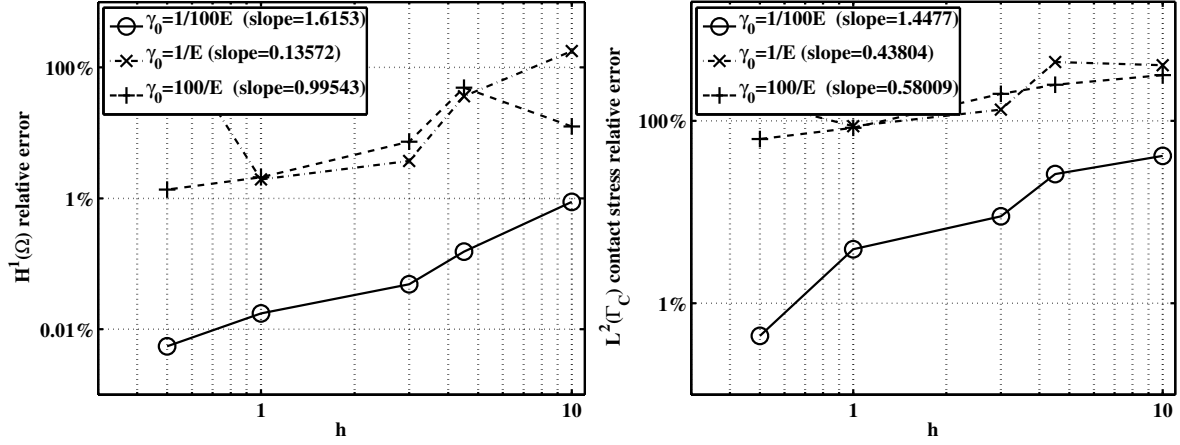
Figure 5: Convergence in the 2D case with P_2 elements and \theta = 1 . Left : relative H^1(\Omega) -norm on the displacements. Right : relative weighted L^2(\Gamma_C) -norm on the contact pressure.
