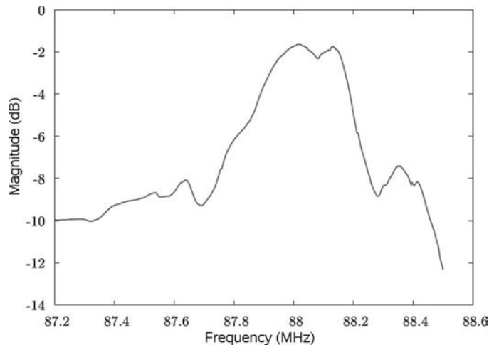
Fig. 9. Transfer function obtained with a filter composed of two rectangular electrodes ( 10\lambda and 20\lambda , respectively) separated by 15\lambda : typical signature of a band-pass filter.
