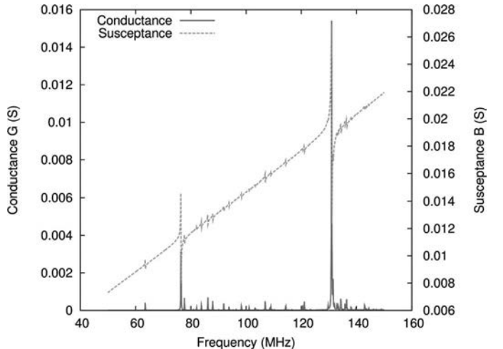
Fig. 3. Theoretical admittance of a 50\text{-}\mu\text{m} -period periodically poled transducer.
