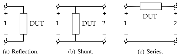
Figure 1. All possible ways to connect a DUT to one and two ports.
