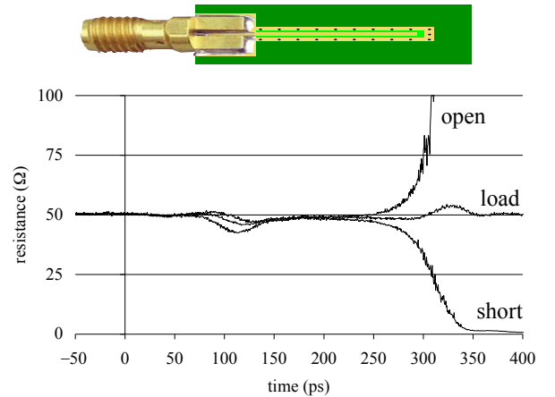
Figure 7. Time domain reflectometry of the short, open and load standards (rise time of 35 ps). The image of the open standard is warped according to ADS LineCalc delay data, t = 0\text{ ps} corresponds with the SMA reference plane.
