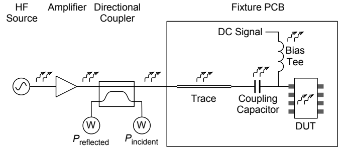
Figure 1. HF injection path of the DPI set-up proposed in IEC 62132-4. The heat waves symbolise lost power. The goal of the set-up is to deliver a known HF power to the IC under test via one particular pin.
