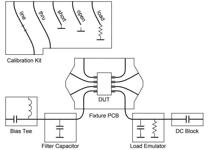
Figure 3. DUT fixture with example periphery. Signal generator and directional coupler not shown.
