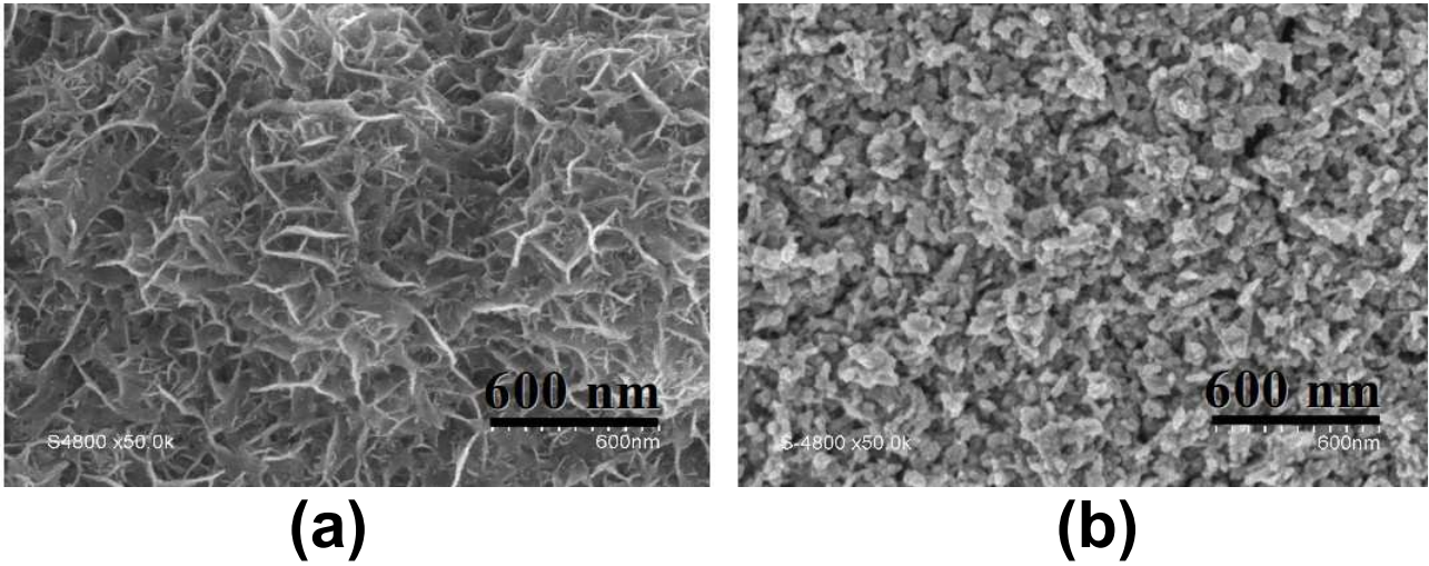
Figure 5 : SEM pictures obtained on \text{In}_2\text{S}_3 films
