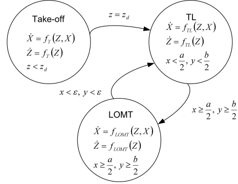
Fig. 5. Navigation control system
