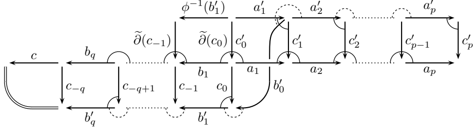
FIGURE 13. Left-division by an element of \mathcal{S}^\sharp starting from a symmetric \mathcal{S} -normal path \overline{b_q} | \dots | \overline{b_1} | a_1 | \dots | a_p .
