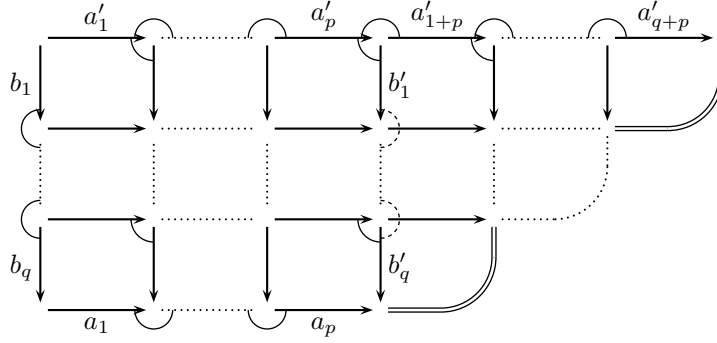
FIGURE 8. Finding an \mathcal{S} -normal decomposition of b_1 \cdots b_q a_1 \cdots a_p when b_1 | \cdots | b_q and a_1 | \cdots | a_p are \mathcal{S} -normal: using Proposition 4.3, hence the first domino rule only, one determines the \mathcal{S} -normal sequence a'_1 | \cdots | a'_{q+p} in pq + q(q-1)/2 steps; if the second domino rule is valid, the sequence b'_1 | \cdots | b'_q is already \mathcal{S} -normal, and a'_1 | \cdots | a'_p | b'_1 | \cdots | b'_q is an \mathcal{S} -normal decomposition of b_1 \cdots b_q a_1 \cdots a_p .
