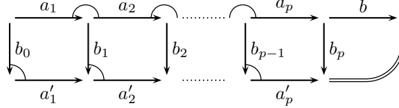
FIGURE 7. Algorithm 4.7: starting from an \mathcal{S} -normal decomposition of g and b , it returns an \mathcal{S} -normal decomposition of gb .
