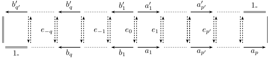
FIGURE 2. Deformation of a signed path by invertible elements: invertible elements connect the corresponding entries; if some path is shorter than the other (here we have q < q' and p' < p ), it is extended by identity-elements.
