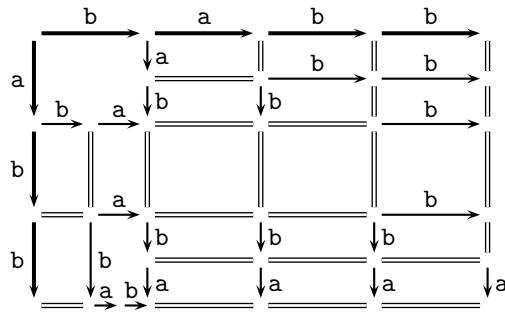
FIGURE 5. The grid associated with a right-reversing for a right-complement that is not short. Here we consider the right-complement \theta on \{a, b\} defined by \theta(a, a) = \theta(b, b) = \varepsilon , \theta(a, b) = b|a , and \theta(b, a) = a|b (with one object only), and apply Algorithm 2.5 to the negative-positive word \bar{b}|\bar{b}|\bar{a}|b|a|b|b (the same as in Figure 3): the difference is that, now, edges of variable size occur, so that, a priori, the process need not terminate. In the current case, it terminates, and the output word is a|b|\bar{a} .
