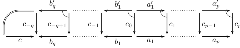
FIGURE 12. Algorithm 5.13: starting from c in \mathcal{S}^\sharp and a symmetric \mathcal{S} -normal decomposition \overline{b}_q | \cdots | \overline{b}_1 | a_1 | \cdots | a_p of g , one obtains a symmetric \mathcal{S} -normal decomposition of cg .
