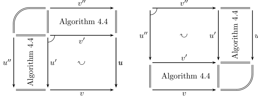
FIGURE 11. Switching normalization and left-reversing in Algorithm 5.5: on the left, we first left-reverse v|\bar{u} into \bar{u}'|v' and then normalize u' into u'' and v' into v'' ; on the right, we first normalize u into u' and v into v' and then left-reverse v'|\bar{u}' into \bar{u}''|v'' .
