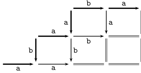
FIGURE 4. The grid associated with the right-reversing of a signed path. We consider the right-complement from Figure 3, and apply Algorithm 2.5 to the word a|\bar{b}|a|\bar{a}|b|a : the initial word is written on the top-left boundary (negative edges vertically and positive edges horizontally), and completing the grid to the bottom-right yields the output word a|a .
