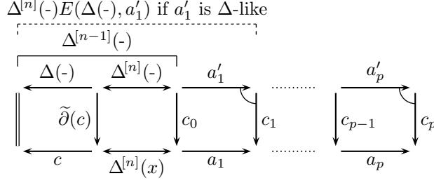
FIGURE 15. Algorithm 5.20 : Computing a \Delta -normal decomposition for c^{-1}g from a \Delta -normal decomposition of g .
