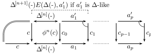
FIGURE 14. Computing a \Delta -normal decomposition of cg starting from a \Delta -normal decomposition of g : the |n| entries of the type \Delta(-) are treated directly using \phi^n , and then it just remains to left-multiply a (positive) \Delta -normal sequence by an element of \mathcal{S} using the standard method. Note that, depending on the sign of n , the diagrams for \Delta^{(n)}(-) consists either of n right-oriented arrows (case n \geq 0 ) or of |n| left-oriented arrows (case n \leq 0 ).
