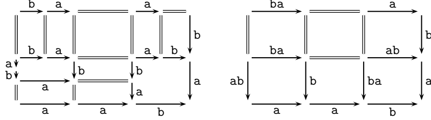
FIGURE 10. Left-reversing of the word a|a|b|\bar{a}|\bar{b} using the left-complement on \{a, b\} (left) and the left-lcm selector on the Garside family \{a, b, ab, ba, \Delta\} (right). Here the right diagram corresponds to gathering pieces of the left diagram, but this would not necessarily be the case for more complicated examples.
