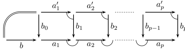
FIGURE 6. Algorithm 4.2: starting from b in \mathcal{S}^\sharp and an \mathcal{S} -normal decomposition of g , it returns an \mathcal{S} -normal decomposition of bg .
