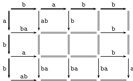
FIGURE 9. The grid associated with the right-reversing of \overline{u|v} in Example 4.18; compare with the grid of Figure 5: the final paths are equivalent, but not equal, which is not contradictory as they are obtained in different ways.
