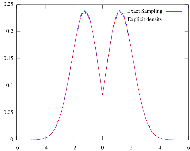
FIGURE 1: Brownian motion with two-valued drift, case \theta_0 = -\theta_1 = 1 ( T = 1 ).
