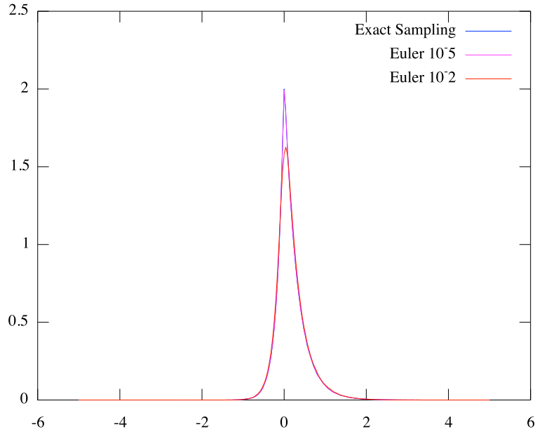
FIGURE 4: Limit algorithm v.s. Euler Scheme for the case where \bar{b} is given by (32) ( x = 0.0 and T = 1 ).
