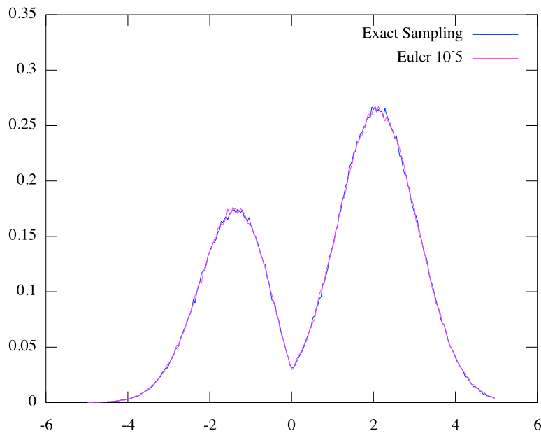
FIGURE 3: Limit algorithm v.s. Euler Scheme for Brownian motion with two-valued drift with \theta_0 = 2 and \theta_1 = -1 ( x = 0.0 and T = 1 ).
