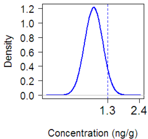
Benzo.a.pyrene
