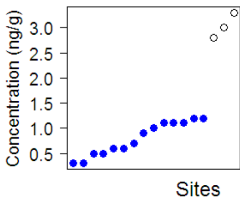
Benzo.a.pyrene
