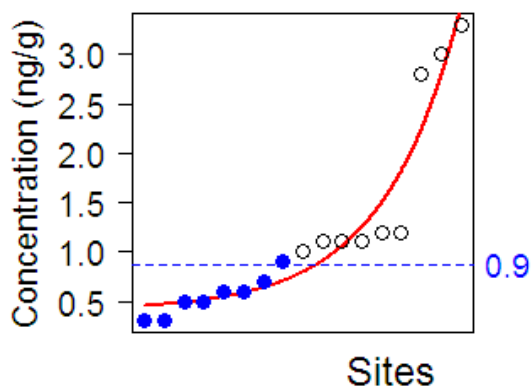
Benzo.a.pyrene
