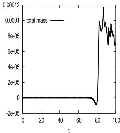
Figure 6: Time evolution of the total mass.
