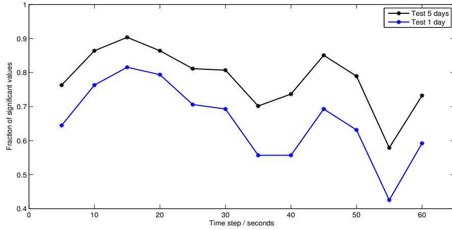
Figure 6: Fraction of the out-of-sample test values that are rejected by the significance test, using the 5% confidence level. Blue stands for the one-day test and black for the five-day test.
