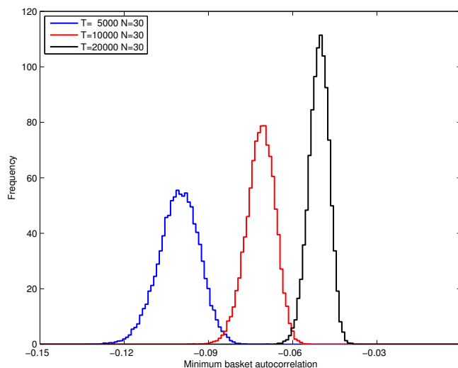
Figure 2: Empirical distribution of the optimal anti-autocorrelation for a basket built from 30 synthetic stock timeseries with i.i.d. normally distributed increments.
