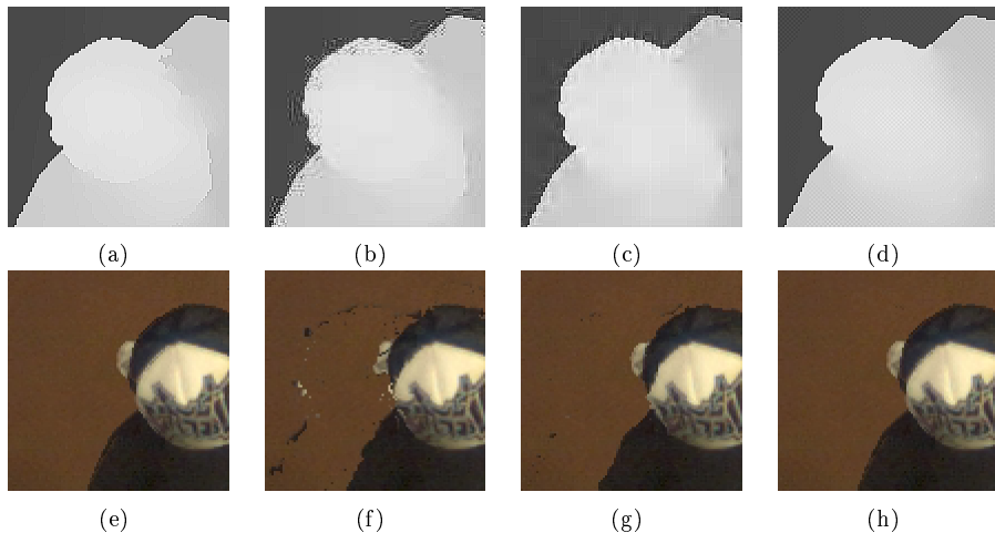
Figure 7: Upper row: zoom on the head of a dancer on original View#3 ( V_3 ) depth map (a) highlights by comparison the ringing artifact on JPEG (b) and JPEG2000 (c). Our method (d) based on exact edges and homogeneous diffusion prevent this effect. (Depth maps have been sharpened for distortion visibility). Lower row: zoom on synthesized view V_4 without (e) or with JPEG (f), JPEG2000 (g) and our method (h) compressions at equal PSNR (43dB) referenced to (e).
