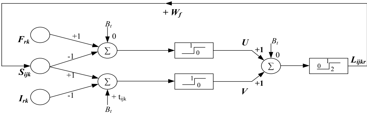
Fig. 4.(a) Hopfield Neural Network for solving an overlapping between a production operation and a maintenance task on machine k
