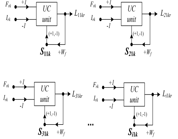
Fig. 5. (c) Construction architecture of unavailability constraints
