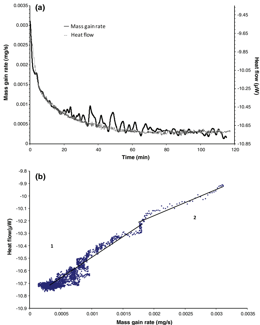
Fig. 3. Cermet oxidation at 960 °C under 2 kPa of oxygen partial pressure: (a) mass gain rate and heat flow vs. time (b) heat flow vs. mass gain rate.
