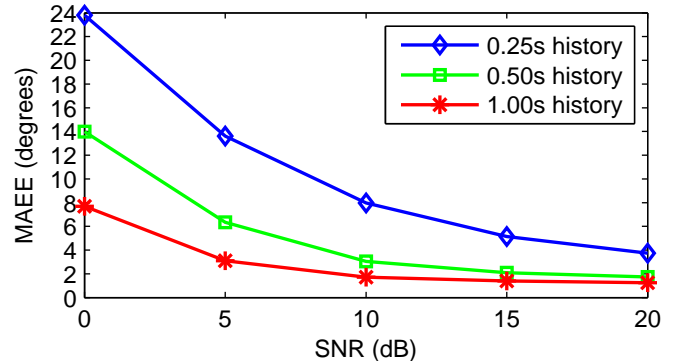
Fig. 5. DOA estimation error vs SNR for four intermittent speakers simulated reverberant environment.
