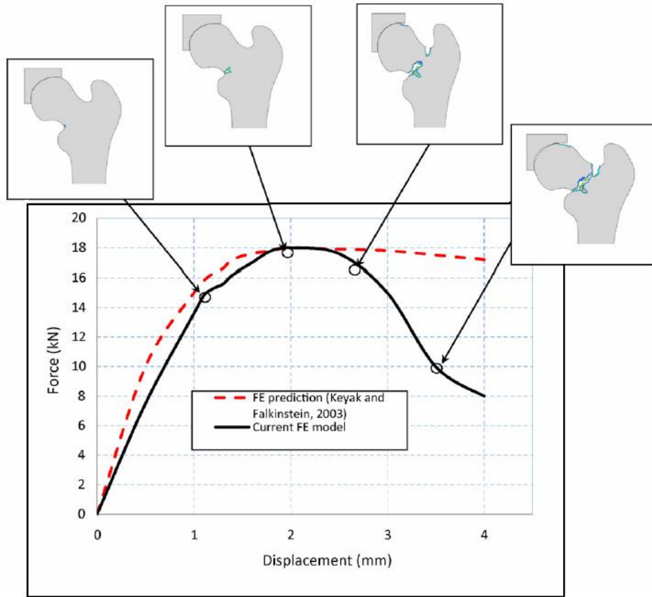
Figure 1. Predicted force–displacement curve obtained by the proposed model, comparison with Keyak and Falkinstein results [8]. The cracks propagation within the proximal femur in relation with the curve is reported. Solid arrows correspond to the profiles sequences related to the brittle bone and dashed arrows correspond to the profiles sequences related to the quasi-brittle bone
