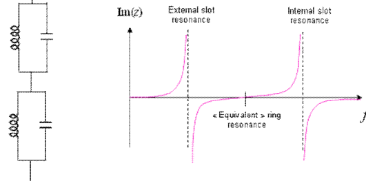
Figure 6. Equivalent electric circuit of the cell
