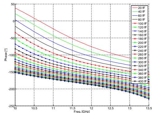
Figure 8. Phase versus frequency for C3 variable, C1 and C2 constant equal to 20fF ( L_C=12\text{mm} , L_P=1.5\text{mm} , W_S=1.425\text{mm} , W_R=1.7\text{mm} )
