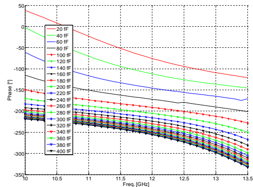
Figure 7. Phase versus frequency for C3 = 20\text{fF} , and simultaneous variation of C1 and C2 ( L_C=12\text{mm} , L_P=1.5\text{mm} , W_S=1.425\text{mm} , W_R=1.7\text{mm} )
