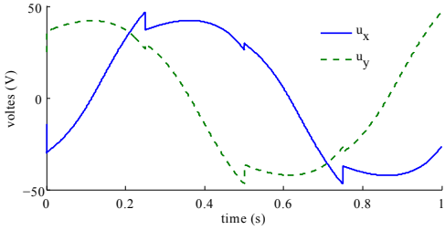
(b) The computed u_x and u_y values for tracking the low speed trajectory.
