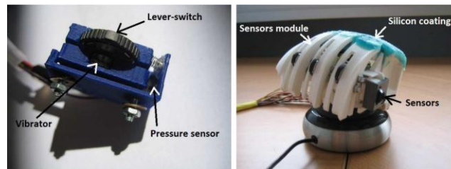
Figure 1. Our new prototype (on the left, a module for one finger).
