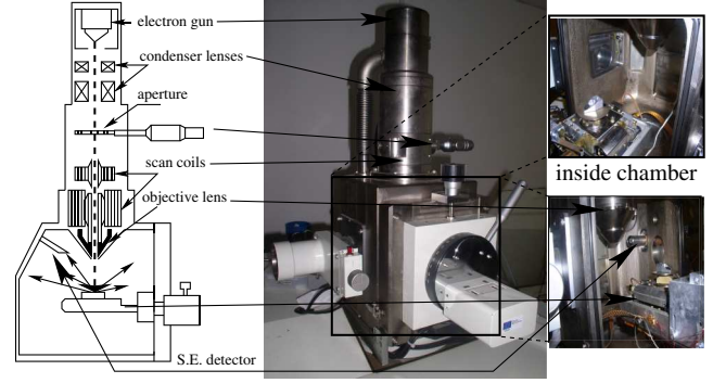
Fig. 7 The JSM 820 SEM manufactured by JEOL.
