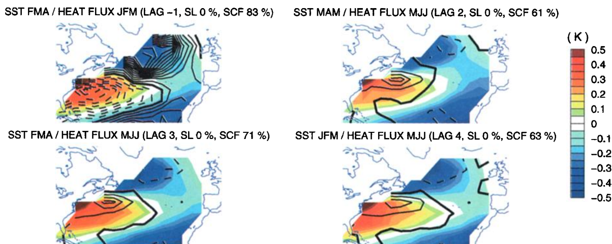
Plate 2. As in Plate 1 but for the surface turbulent heat flux (positive upward, contour 3 \text{ W m}^{-2} ) instead of Z500. Lag 0 and 1 are not represented.
