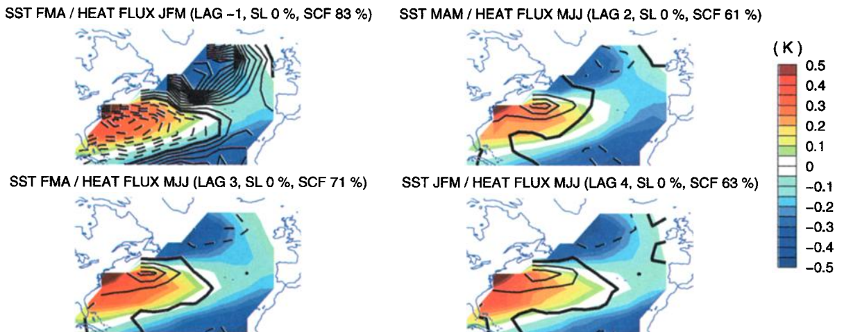
Plate 2. As in Plate 1 but for the surface turbulent heat flux (positive upward, contour 3 Wm^{-2} ) instead of Z500. Lag 0 and 1 are not represented.
