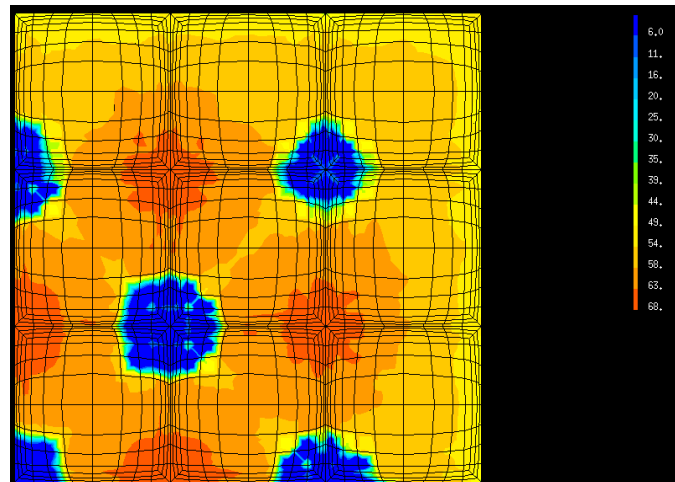
Figure 6 : Concentration after diffusion in a transversal section \text{UO}_2 -side.
