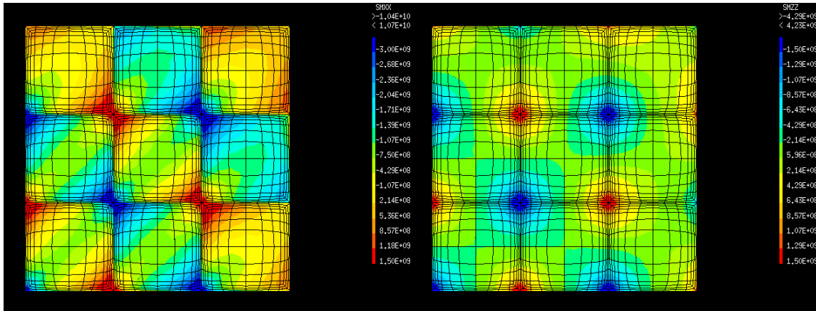
Figure 5 : \sigma_{11} and \sigma_{33} stresses on a section parallel to the \text{UO}_2/\text{U}_3\text{O}_7 interface at 1 nm depth inside \text{UO}_2 .
