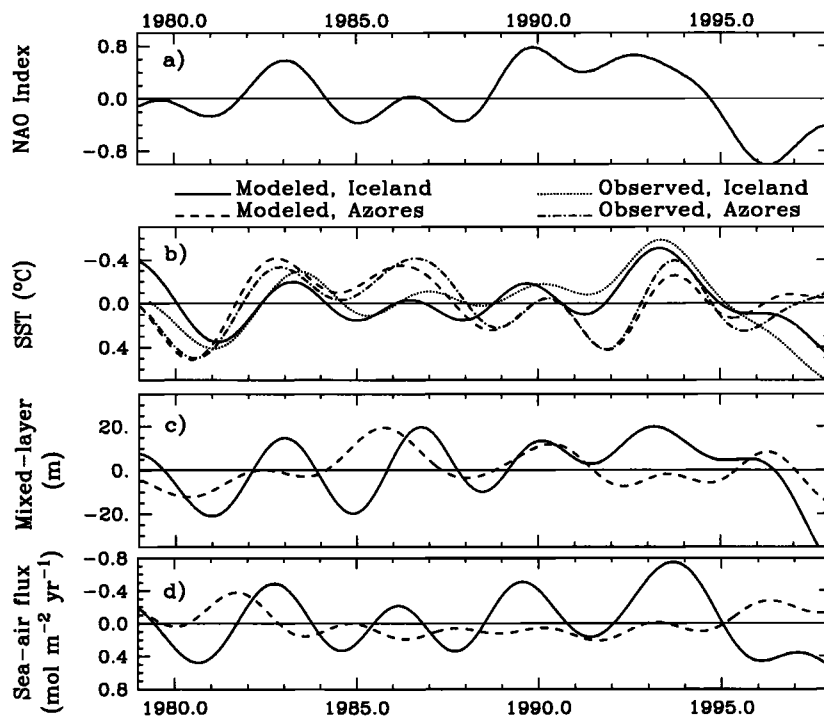
Figure 4. Interannual anomalies in the North Atlantic of (a) the North Atlantic Oscillation (NAO) index [Hurrell, 1995], (b) the modeled and observed SST ( ^{\circ}\text{C} ) [Reynolds and Smith, 1994], (c) the mixed layer depth (m), and (d) the sea-air flux ( \text{mol m}^{-2} \text{yr}^{-1} ). The solid lines in figures 4b-4d are results at station India, near Iceland ( 59^{\circ}\text{N} , 19^{\circ}\text{W} ); dashed lines are results for the Azores ( 39^{\circ}\text{N} , 28^{\circ}\text{W} ). The data and model results are filtered to remove frequencies above 1 \text{ year}^{-1} [Thoning et al., 1989]. The axis for the SST and CO 2 flux were reversed to illustrate their relationship with the NAO.
