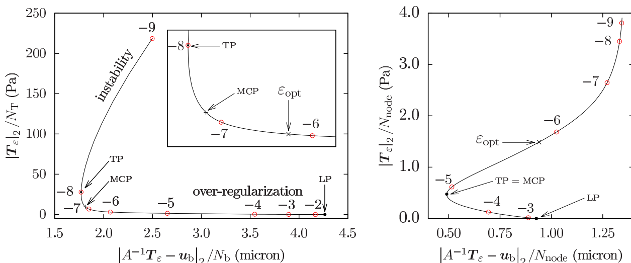
Figure 3 – L -curves obtained using the adjoint method (left) and p-FTTC (right). Mechanical parameters: E = 10 kPa and \nu = 1/2 . Data : N_b = 3,144 beads. Mesh used by the adjoint method: 9,323 nodes, N_T = 1,109 nodes in \Omega_c and 18,332 triangles, P_1 interpolation. Spatial grid used by the p-FTTC method: 256 \times 256 nodes ( N_{\text{node}} = 65,536 ), N_T = 6,396 nodes in \Omega_c . Some values of the decimal logarithm of \varepsilon are reported on the graphs (red circles). TP: turning point. MCP: maximum curvature point. LP: limit point. \varepsilon_{\text{opt}} : optimal value of the regularization parameter used in Fig. 4, 5 and 6.
