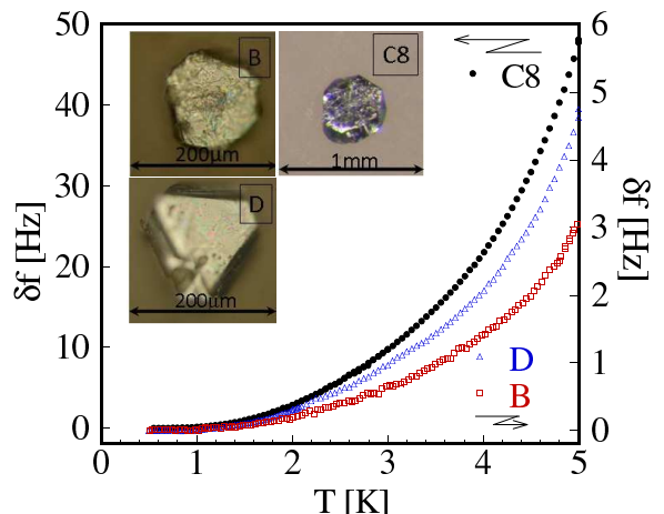
Figure 1: Temperature dependence of the frequency shift \delta f(T) , for B (square) D (triangle) (right scale) and C8 (circle) (left scale) NbS 2 single crystals. Inset: microscope images of each sample (note the bigger scale for C8).
