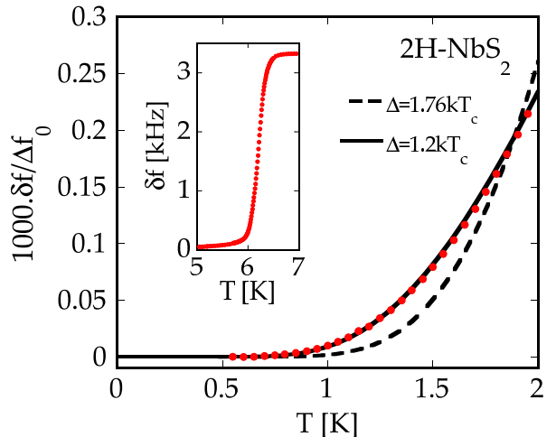
Figure 2: Temperature dependence of the rescaled frequency shift \delta f/\Delta f_0 \propto \Delta \lambda_{ab}/\lambda_0 in NbS 2 at T < T_c/3 (red circles). Results are fitted with the exponential low temperature approximation (see text) to determine the smaller gap \Delta . An excellent fit is obtained for \Delta \approx 1.17 k_B T_c . Results can't be described by an exponential behaviour with the weak coupling BCS value \Delta = 1.76 k_B T_c . Inset: superconducting transition: T_c = 6.05 K is determined by the maximum of variation of the frequency shift.
