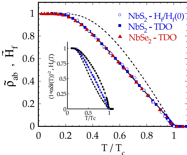
Figure 3: Normalized superfluid density of NbS_2 deduced from Tunnel Diode Oscillator measurements (TDO) for R\lambda_0/\Delta f_0=0.02Hz^{-1} (closed squares), compared to H_f(T)/H_f(0) (open circles) both on sample C8. As shown, the weak coupling BCS normalized superfluid density (dashed line) is not compatible with the data. A very similar temperature dependence was previously obtained in NbSe_2 (solid triangles) and both compounds could be well described by a two gap model (thick line, see text for details). Inset: influence of the R/\lambda_0\Delta f_0 parameter on the shape of the superfluid density, R/\lambda_0\Delta f_0 being equal to respectively 0.01, 0.02 and 0.03 Hz^{-1} for diamonds, squares and circles.
