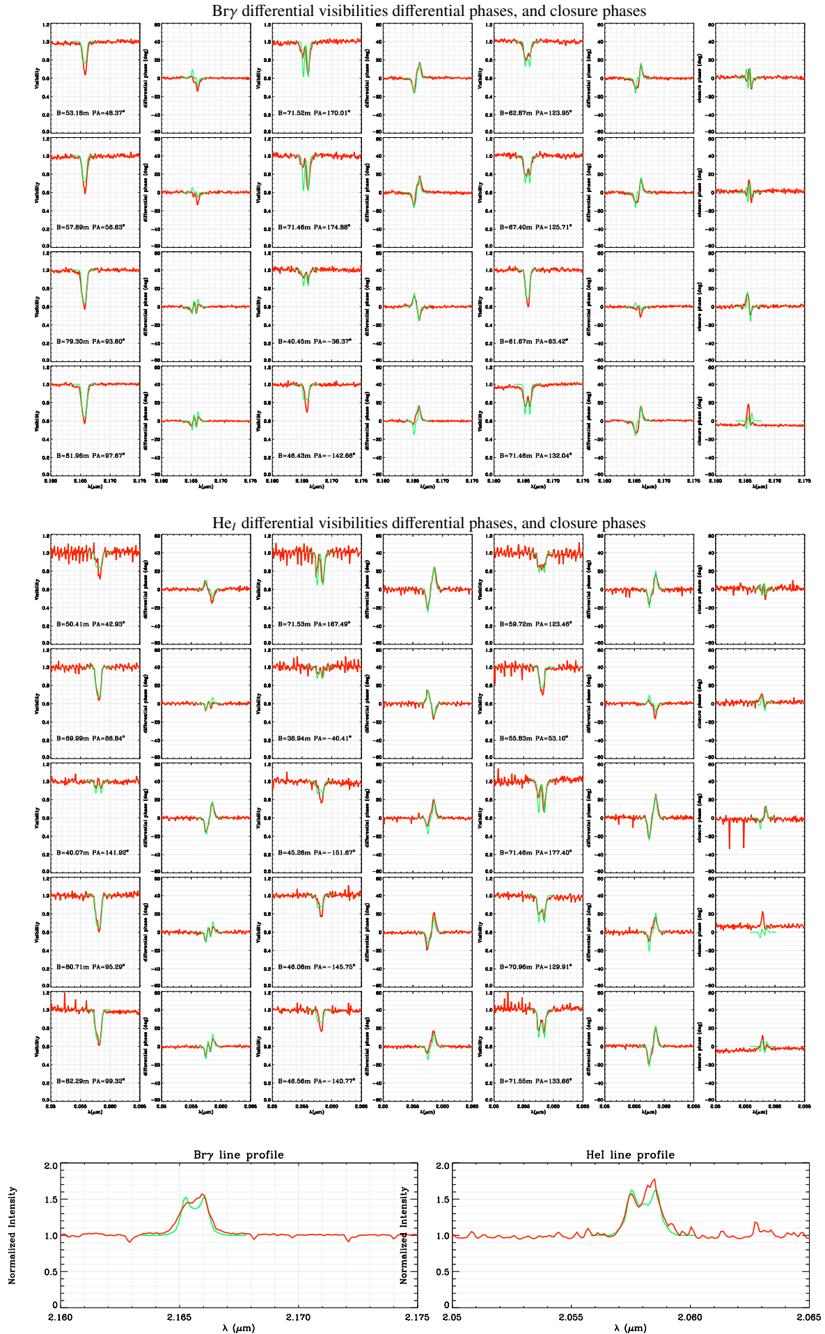
Fig. 3. The full dataset for \delta Sorspii 2012 VLTI/AMBER observations. The red lines represents the VLTI/AMBER data, and the green ones, the best-fit symmetric kinematic model.
