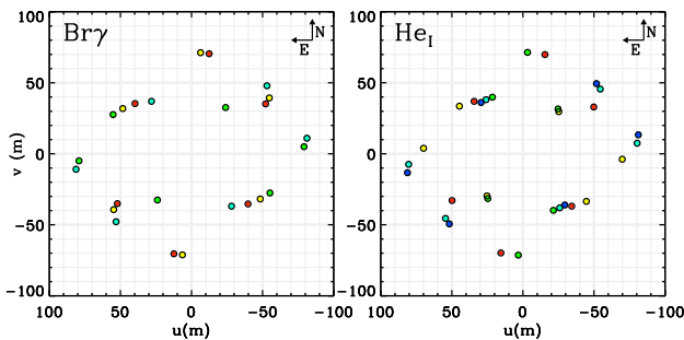
Fig. 1. \delta Scorpii (u,v) 49lan coverage obtained in 2012 with VLTI/AMBER observations centered on Bry (left) and 2.06 \mu\text{m} He I (right) emission lines.
