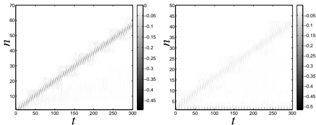
Figure 4: Space-time diagrams showing the interaction forces f_n = -(y_n - y_{n+1})_+^{3/2} in system (2) with \gamma = 1 and free end boundary conditions. Forces are represented in grey levels, white corresponding to vanishing interactions (beads not in contact) and black to a minimal negative value of the contact force. The initial condition is y_n(0) = 0 for n \geq 1 , \dot{y}_n(0) = 0 for n \geq 2 , \dot{y}_1(0) = 0.94 . For a harmonic local potential ( s = 0 , left plot), a traveling breather is generated. For a soft local potential ( s = -0.7 , right plot), one observes in addition the excitation of a surface mode.
