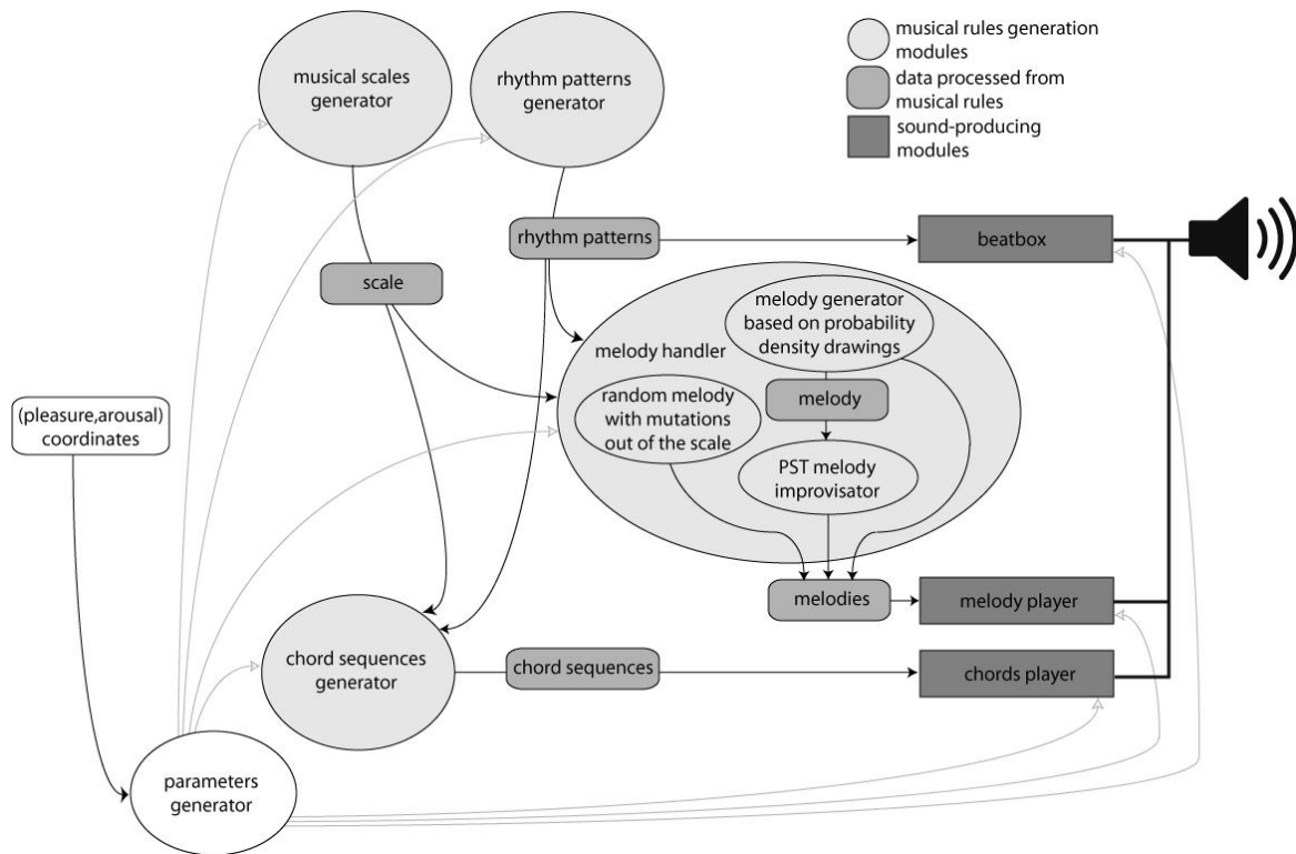
Figure 2: Musical rules generation modules: MuZICO
