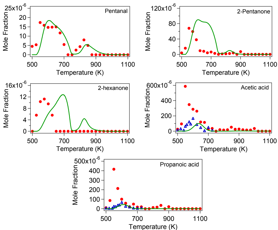
Figure 5: Mole fractions of C 1 -C 6 oxygenated products (Part II). ●: Experimental results obtained in Nancy. △: Experimental data obtained in Hefei (mole fractions of organic acids were calculated from the SVUV-PIMS signals obtained for m/z 60 and 74 at 11 eV). —: Simulation.
