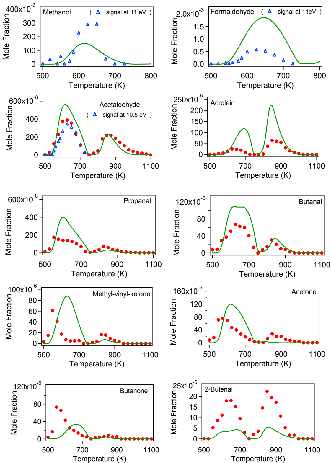
Figure 4: Mole fractions of C 1 -C 6 oxygenated products (Part I). ●: Experimental results obtained in Nancy. △: Experimental data obtained in Hefei (mole fractions of methanol and formaldehyde were calculated from the signals obtained at 11 eV and the one of acetaldehyde from the signal obtained at 10.5 eV). —: Simulation.
