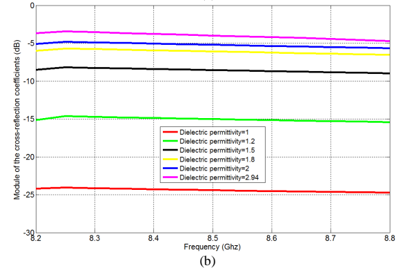
Figure 7. Amplitude of the (a) RHCP/LHCP transmission coefficient, (b) Cross-reflection coefficient for various permittivity values. In all cases, the dielectric spacer is 8mm-thick.
