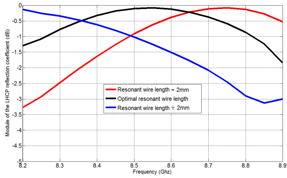
Figure 9. Module of the LHCP reflection coefficient for three resonant wire lengths.
