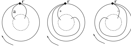
FIGURE 10. a, a^+, a^-
