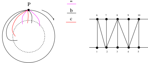
FIGURE 14. Simplicial relations between f^{-1}([b]) and f^{-1}([c])
