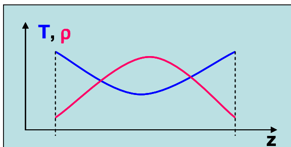
Figure 2: Temperature and the particle distributions in the cell containing a gas in thermodynamics equilibrium and evolving according to the model of § - 4.b, that is in which one extracts locally a heat proportional to the local energy of the local collisions
