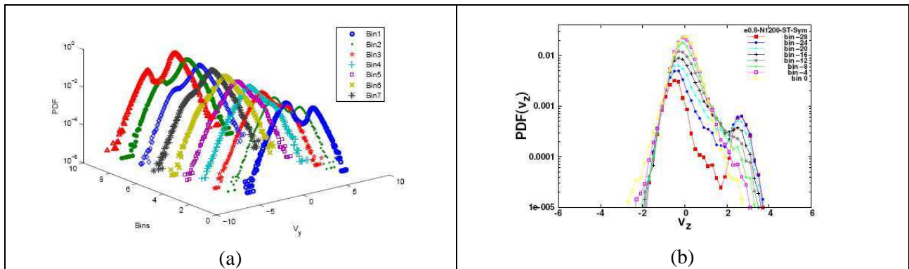
Figure 5: Local speed distributions V_z in the cell as a function of the z position ( Oz is // to vibration). (a) : 2d case ; (b) : 3d case, in the left-hand half cell. [2,4,13.b]
