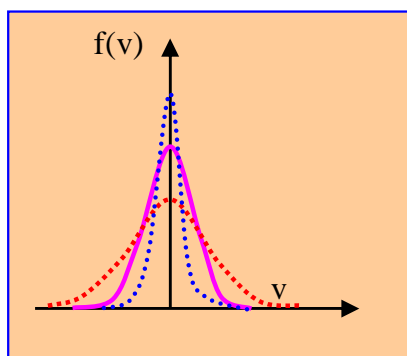
Figure 3: Local distribution of the speeds of particles in the model of § - 4.b. The three curves represent various places, at different temperatures of gas (blue at the cell centre, purple at a distance of a quarter cell from the wall, red in the edge). The distribution which dominates in high speed is the broadest corresponding to the highest temperature.
