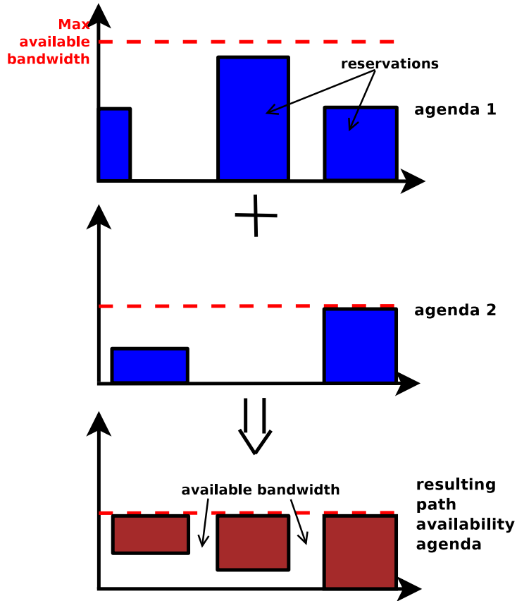
Figure 8: Agenda fusion
