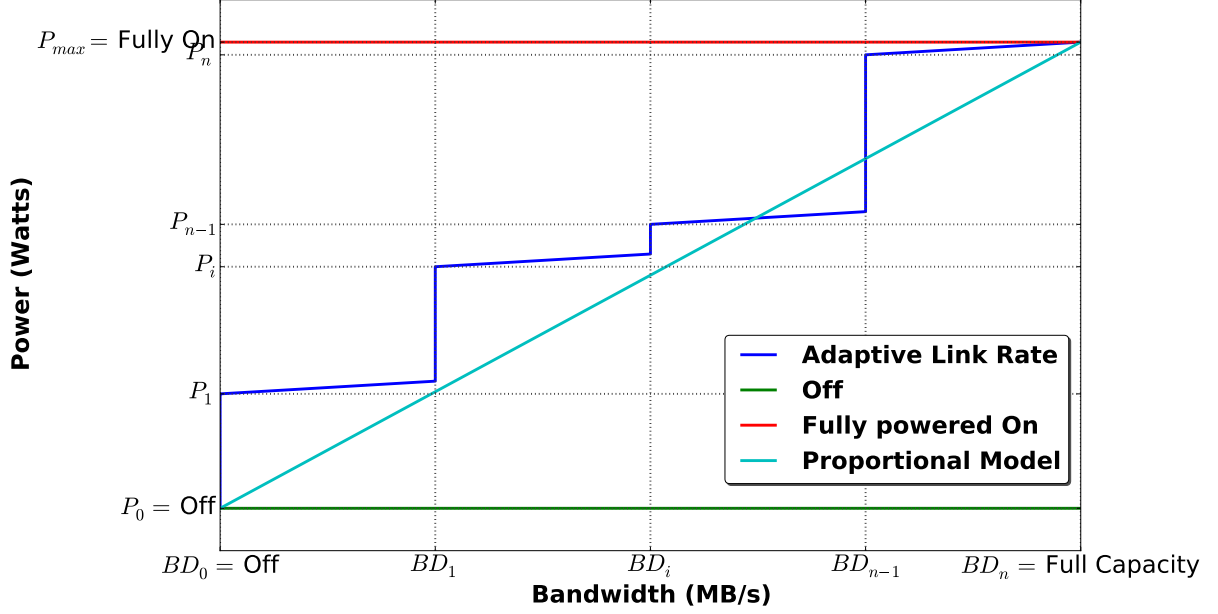
Figure 1: Models of power cost as a function of bandwidth
