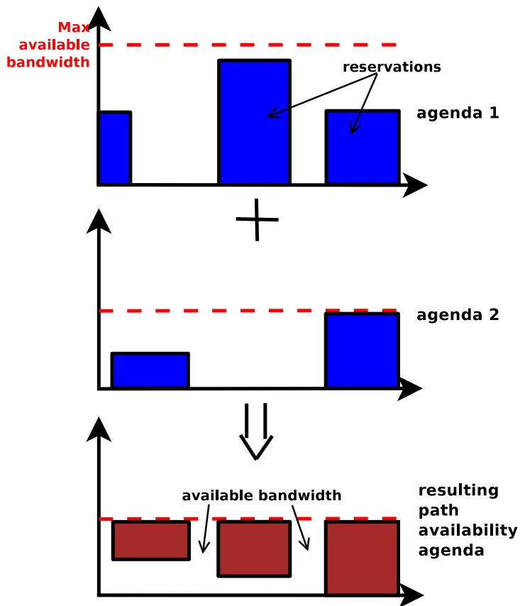
Figure 8: Agenda fusion
