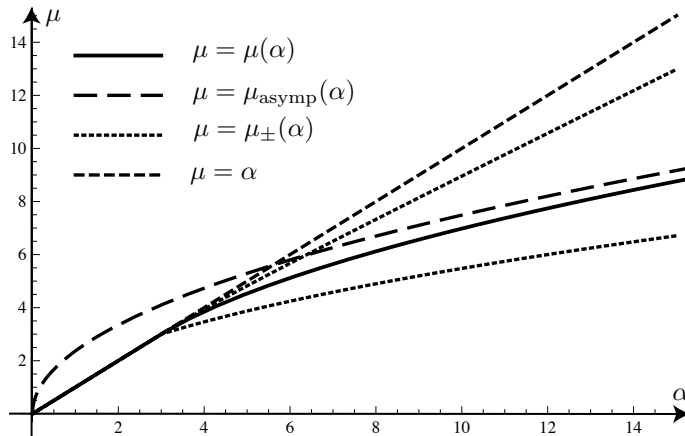
FIGURE 1. In the case q > 2 , the optimal constant is given by \mu = \alpha for \alpha \leq d/(q-2) and the curve \mu = \mu(\alpha) for \alpha > d/(q-2) . An upper estimate is given by the curve \mu = \mu_+(\alpha) obtained by optimizing the function h_\alpha(\varepsilon) in terms of \varepsilon \in (0, 1) while a lower estimate, namely \mu = \mu_-(\alpha) = \alpha_*^\vartheta \alpha^{1-\vartheta} has been established in Proposition 8. The asymptotic regime is governed by \mu(\alpha) \sim \mu_{\text{asyp}}(\alpha) = K_{q,d} \kappa_{q,d}^{-1} \alpha^{1-\vartheta} as \alpha \rightarrow +\infty according to Lemma 5. The above plot shows the various curves in the special case d = 3 and q = 3 .
