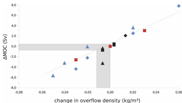
FIG. 4. Sensitivity of the MOC (Sv) to changes in the potential density \sigma_0 ( \text{kg m}^{-3} ) of the Denmark Strait overflow obtained from simulations using two global ocean models (ORCA2 and ORCA05) with horizontal resolutions near 60^\circ\text{N} of 120 (blue) and 30 (black) km, and an Atlantic model (FLAME) with a horizontal resolution of 18 km (red). With each of these models a sequence of experiments was performed addressing the response to imposed changes in the hydrographic conditions in the Nordic Seas. The data points depict the evolution of the overflow density at the sill, and the concomitant response of the maximum MOC transport (near 40^\circ\text{N} ) in the North Atlantic, after 15 (square symbol), 30 (diamonds), and 50 (triangles) yr of integration, relative to reference states that correspond to MOCs of 16–18 Sv for the different model versions. According to the model simulations, the estimated decline of the overflow density based on hydrographic observations during the last 30 yr (indicated by the gray bar) would correspond to a slackening of the MOC by about 1 Sv.
