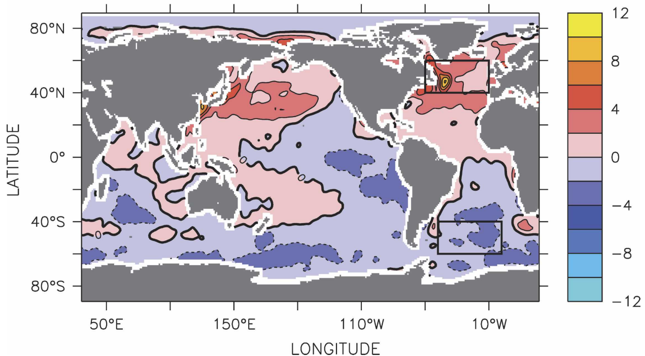
FIG. 1. Linear trend in SST ( ^{\circ}\text{C century}^{-1} ) observed during the period of 1980–2004. The global mean trend was removed to highlight the dynamical changes in the presence of global warming. A clear interhemispheric dipole is seen in the Atlantic, which can be used as a fingerprint to detect changes in the MOC. The two boxes indicate the regions used to define the dipole SST anomaly index shown in Fig. 2.
