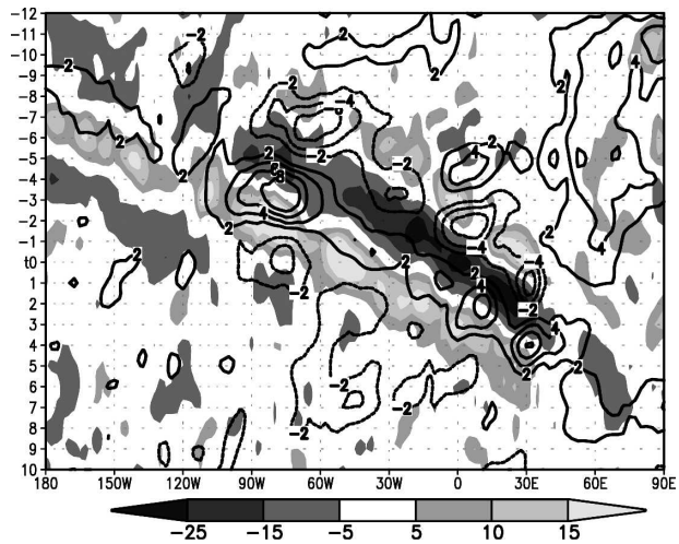
FIG. 5. Composite time–longitude diagram based on the Kelvin wave index for the period June–September 1979–2000. From this standardized index time series, we retained the dates (called t_0 ) when it is maximum (minimum) and greater (lower) than 1.5 to define a dry (wet) Kelvin phase. The respective wet-minus-dry composite sequences have been computed for the nonfiltered OLR (shaded, \text{W m}^{-2} ) and nonfiltered MSLP (contours, hPa) averaged over the latitudes 7.5^\circ\text{--}12.5^\circ\text{N} . This Hovmöller diagram goes from t_0 - 12 days to t_0 + 10 days over the domain 180^\circ\text{--}90^\circ\text{E} .
