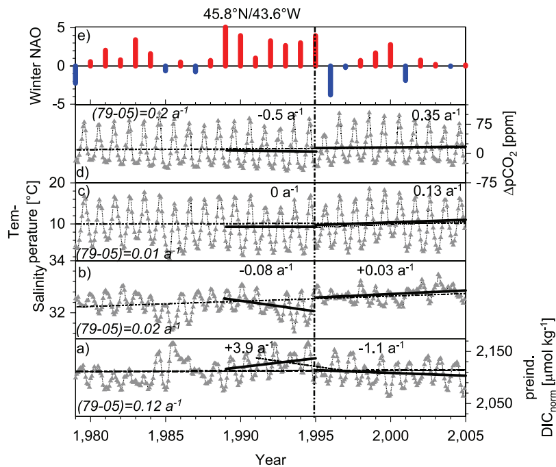
Figure 9. Multiannual variability of preindustrial \text{DIC}_{\text{norm}} , salinity, temperature, and sea-air \Delta p\text{CO}_2 at a western subpolar gyre location. (a) Preindustrial \text{DIC}_{\text{norm}} , (b) salinity, (c) temperature, and (d) sea-air \Delta p\text{CO}_2 at 45.8^\circ\text{N}/43.6^\circ\text{W} . (e) Wintertime North Atlantic Oscillation (NAO) index. Regressions have been performed for the positive NAO period 1989–1995 and the neutral or negative NAO period 1995–2004. The regressions for the entire period 1979 until 2004 are given in italics and by the dotted lines. For comparison with Figures 6 and 7, the slopes of the \text{DIC}_{\text{norm}} regression line for the period 91–96 (shown) are -4.2 \mu\text{mol} (\text{kg a})^{-1} and -0.98 \mu\text{mol} (\text{kg a})^{-1} for the 97–04 period (not shown), respectively.
