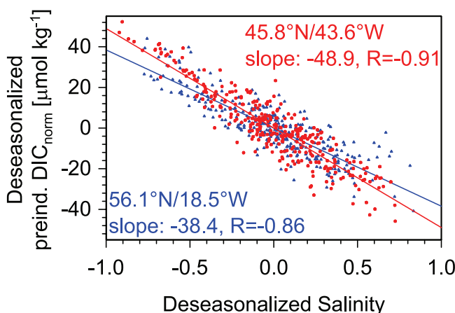
Figure 10. Deseasonalized, preindustrial DIC norm versus deseasonalized salinity for the eastern and western subpolar gyre stations. The red symbols and letters denote the western station at 45.8°N/43.6°W. The blue symbols and letters denote the eastern location at 56.1°N/18.5°W. The contribution from the Labrador Current to the resulting water mass increases in the low-salinity/high-DIC norm direction. The contribution of North Atlantic Current increases in the high-salinity/low-DIC norm direction, respectively. The slopes of the regression lines are given as \mu\text{mol kg}^{-1} (salinity unit) -1 . See Figure S3 for additional information.
