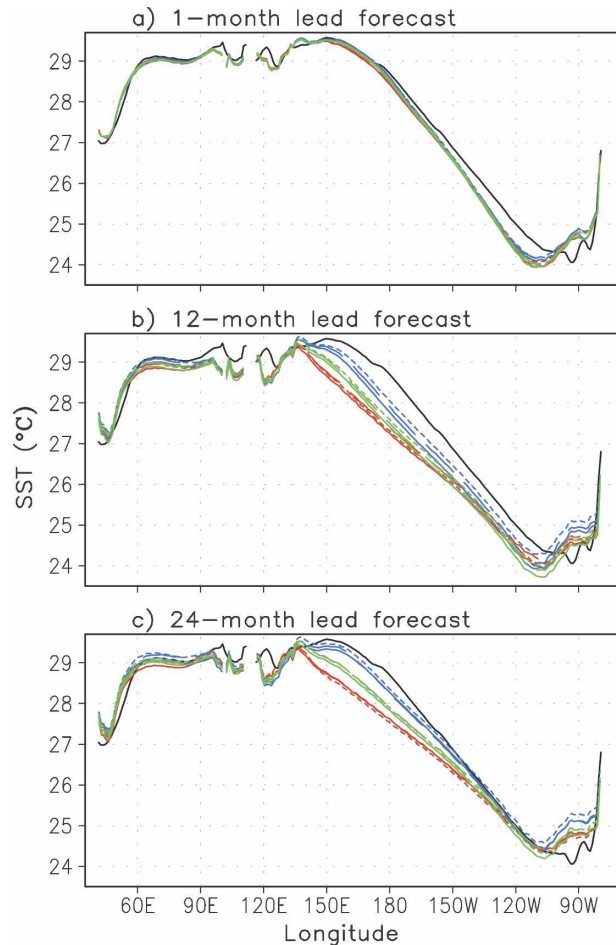
FIG. 1. SST climatology averaged along the equator ( 2^\circ\text{S} – 2^\circ\text{N} ) during the period 1983–2004 based on the NCEP SST observations (black lines) and model predictions (colored lines) at 1-, 12-, and 24-month leads. Climate drifts during the retrospective forecasts in the equatorial Pacific are largely reduced by passing ocean current momentum to the atmosphere (blue curves), compared to the model in which the ocean surface is stationary (red curves). Green lines are produced by the model in which ocean current is taken into account for wind stress calculations but ocean surface is still assumed stationary for the atmosphere. Details for the three models with different coupling physics can be found in Luo et al. (2005a).
