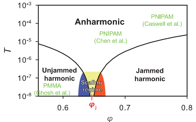
FIG. 12: An enlarged view of the ( T , \varphi ) phase diagram reporting the critical regimes shown in Fig. 8, and the approximate location of the experimental studies aimed at studying anomalous vibrational dynamics in colloidal systems: Gosh et al. [9] use PMMA hard spheres, while Chen et al. [11] and Caswell et al. [15] study PNIPAM microgel particles. Previous studies all lie too far away from the jamming transition to detect the dynamic criticality associated to the transition.
