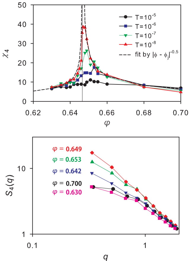
FIG. 5: Top: Volume fraction dependence of the dynamic susceptibility \chi_4(t = t^*) , Eq. (22), for various temperatures showing the emergence of ‘vibrational heterogeneity’ at low enough T close to \varphi_J (shown with the vertical line). Bottom: Four-point correlator S_4(q, t = t^*) at T = 10^{-8} and various volume fractions exhibits a nonmonotonic density dependence (note the nonmonotonic evolution of the \varphi labels).
