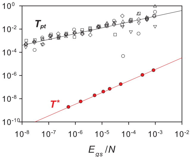
FIG. 10: The crossover temperature scale for the onset of anharmonicity T^* (bottom data with filled circles) compared to the temperature scale T_{\text{pt}} (top data with open symbols different symbols for different packings) quantifying the relevance of the high order terms in the perturbative expansion of the energy. The lines indicate T^* \propto E_{\text{gs}} and T_{\text{pt}} \propto E_{\text{gs}}^{1/2} . Clearly, these two temperature scales differ.
